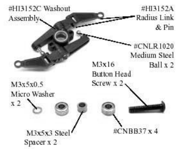
#HW6192A Lower Linkage Set (8 rods)
